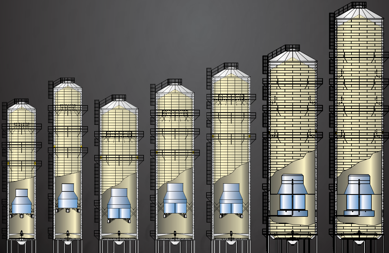
Z-4036 18' dia. x 96'-0" h. 25' dia. w/ Catwalks
